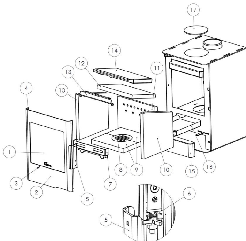
Figure n°7 - Despiece NOMAD
