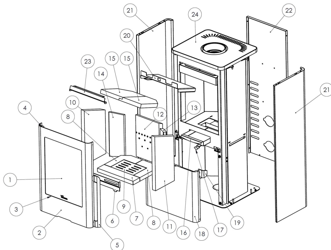
Figure n°1 - Despiece VELA
