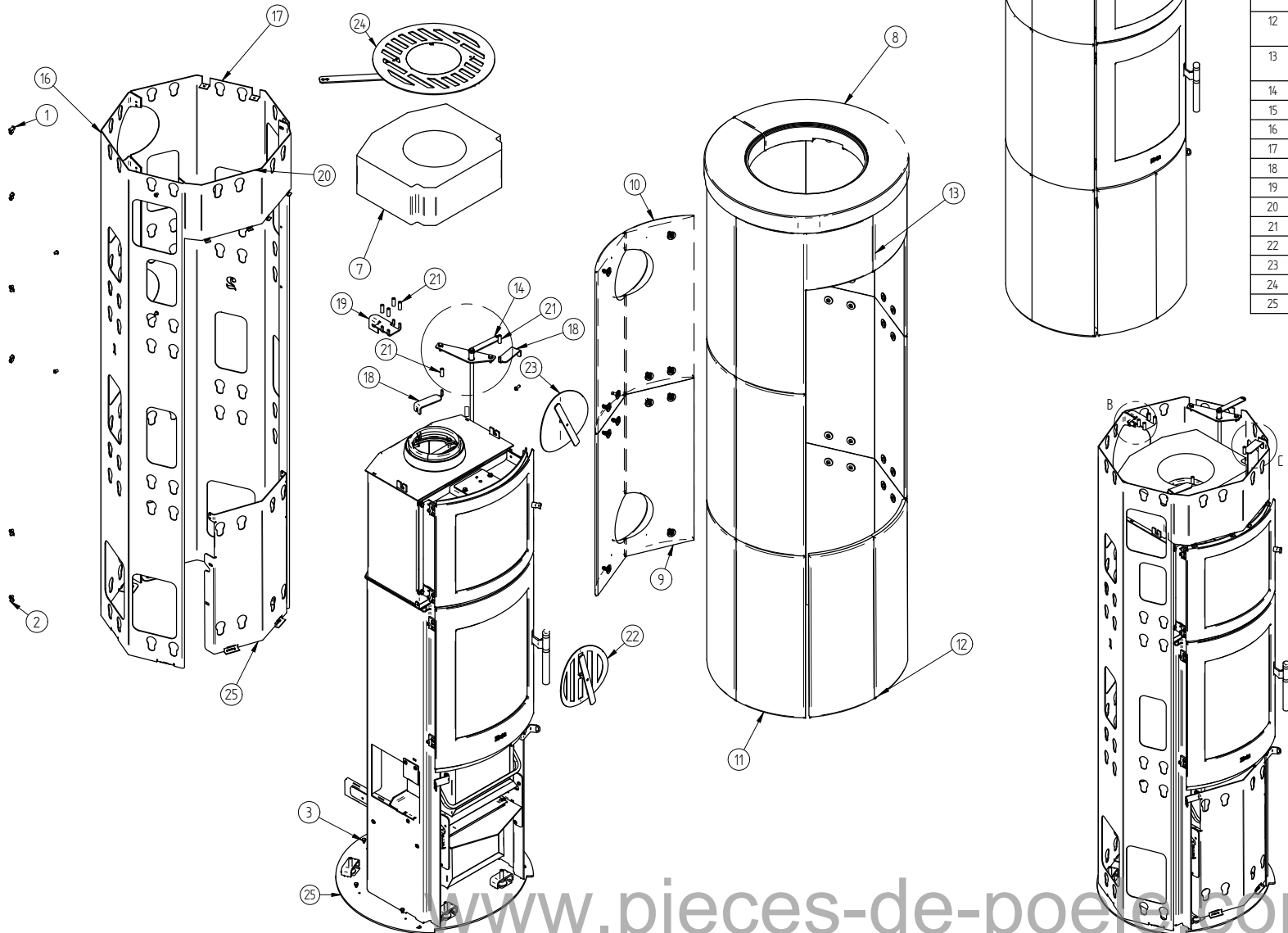
DETAIL D
