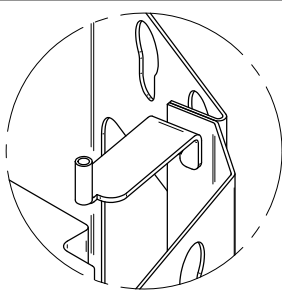
DETAIL C
